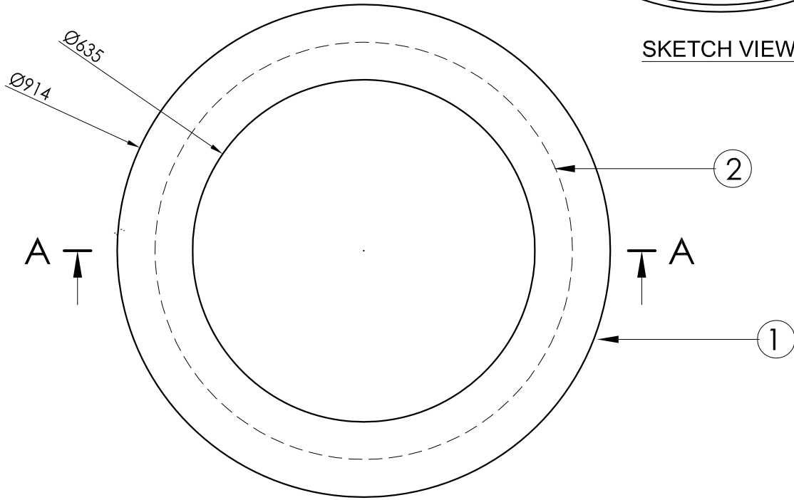
PLAN VIEW SCALE : 1:10
