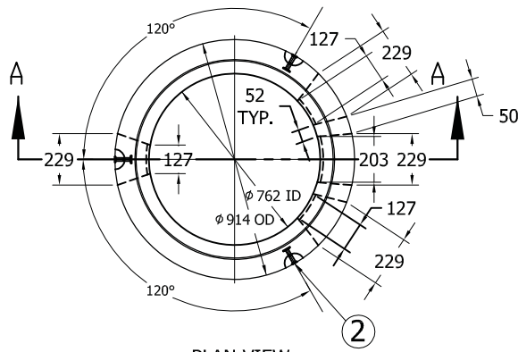
PLAN VIEW SCALE 1:30
