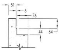
TONGUE & GROOVE DETAIL SCALE 1:15
