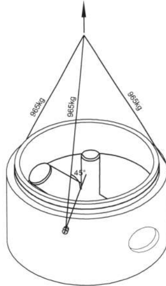
Lifting Detail
