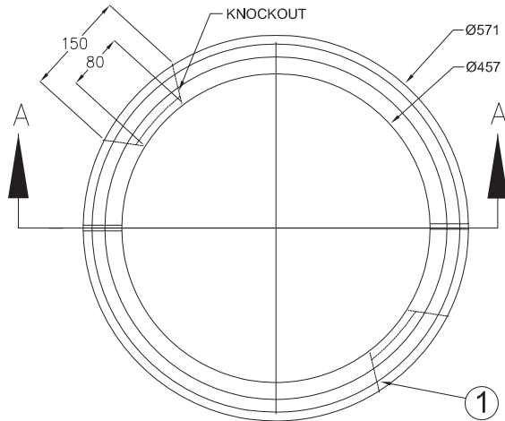
PLAN VIEW SCALE 1:10
