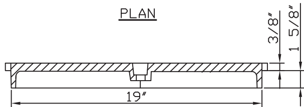
SEC 'A-A'
