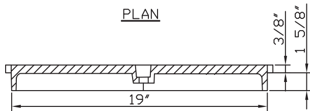
SEC 'A-A'
