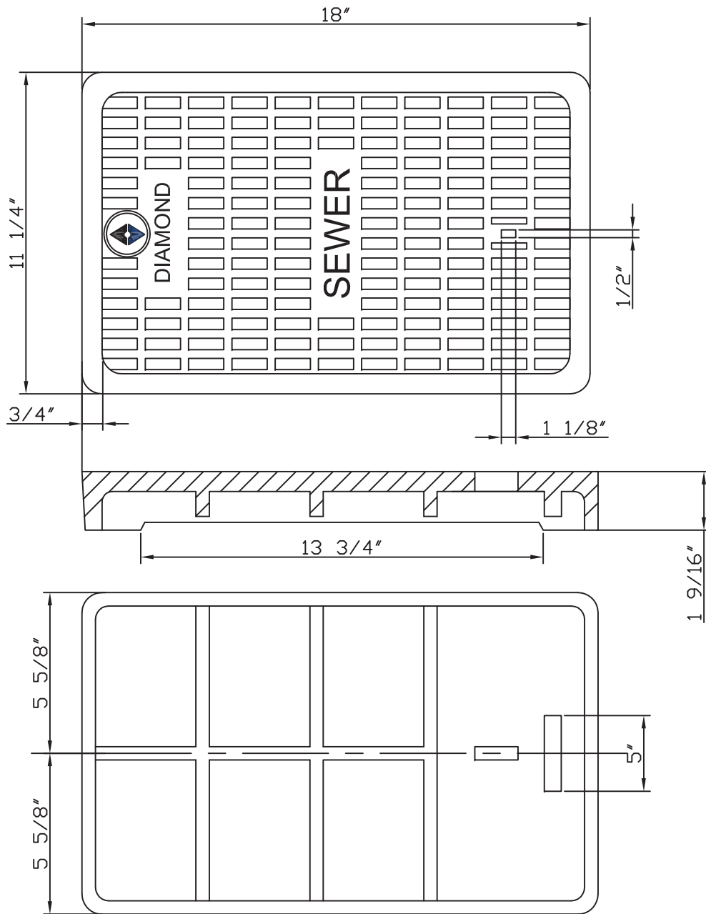
D1811:-Meter Box # 37 Cast Iron Cover-"Sewer"
