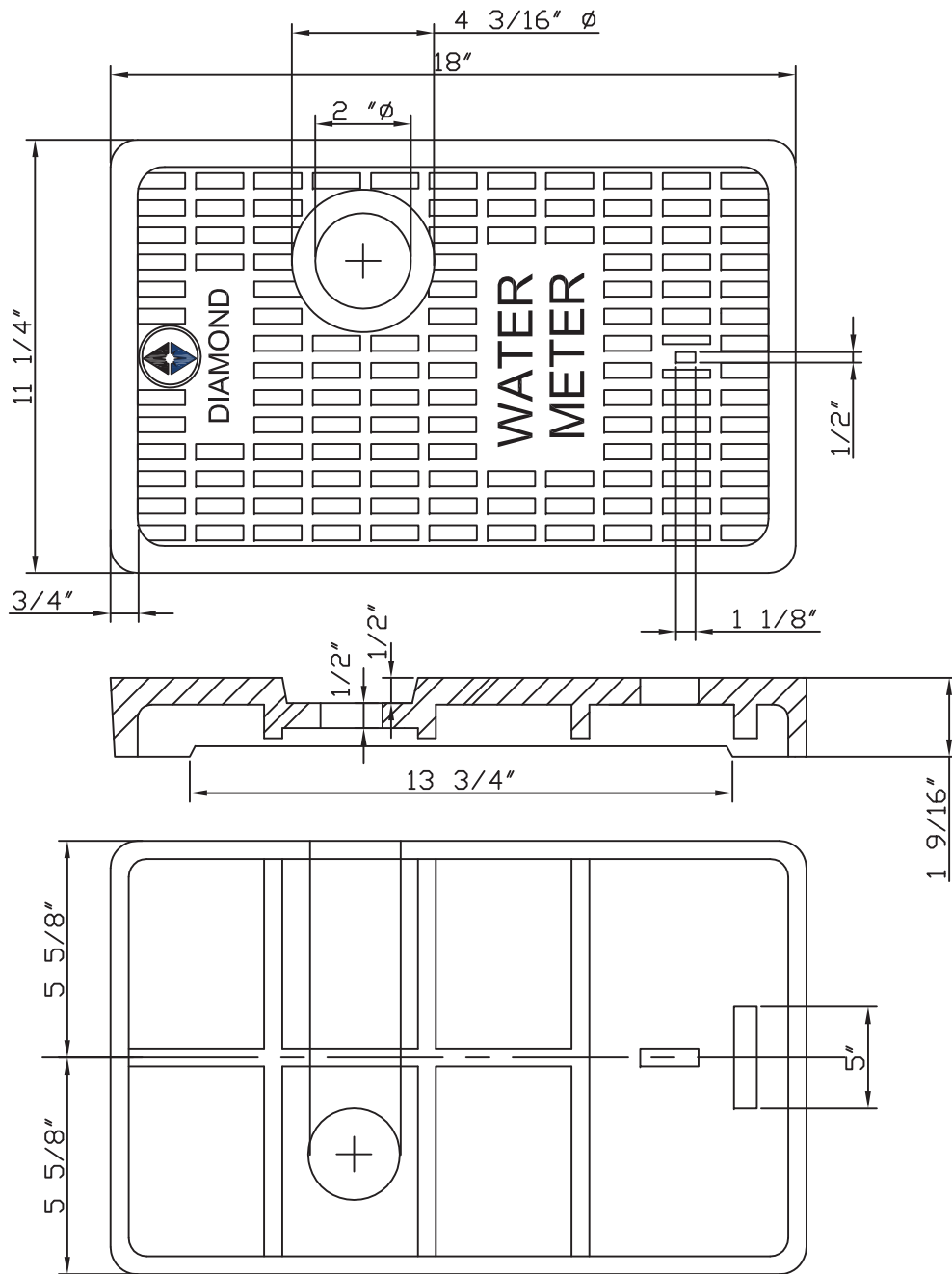
Meter Box # 37 Cast Iron Cover--Hole 23 #
