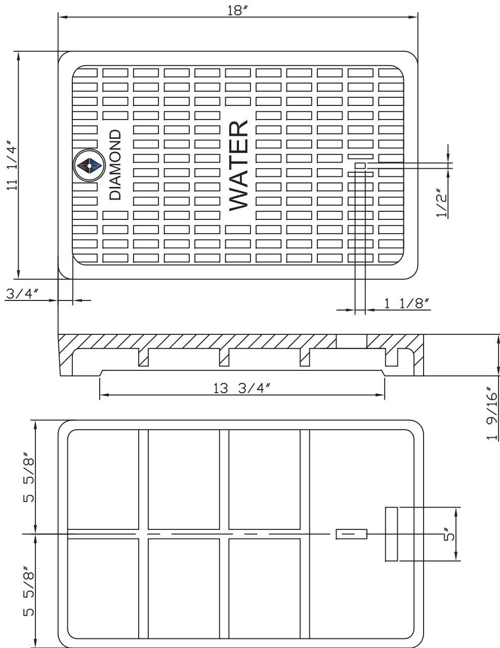
D1811:-Meter Box # 37 Cast Iron Cover-"Water"
