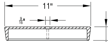
SECTION B - B
