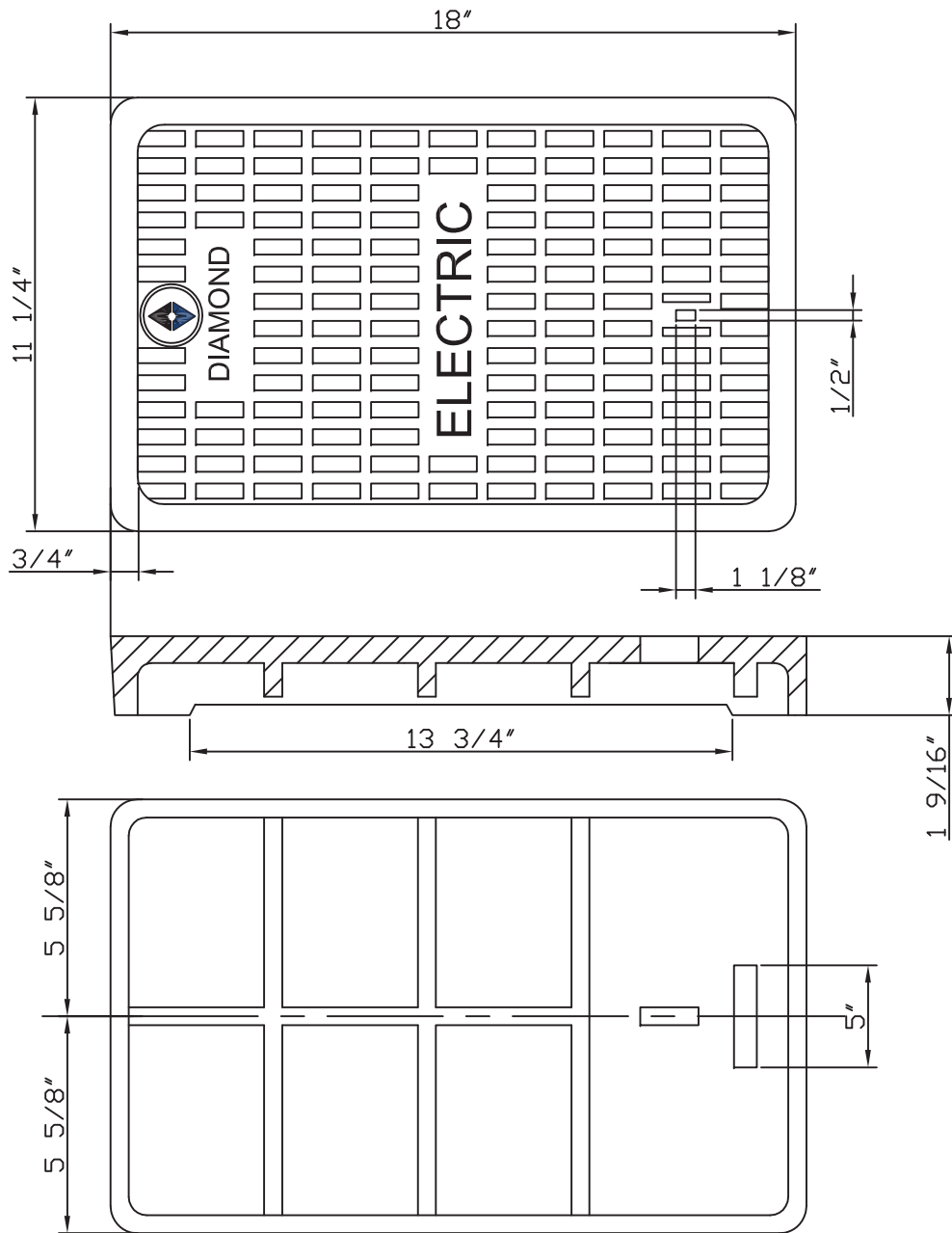
D1811:-Meter Box # 37 Cast Iron Cover-"Electric"
