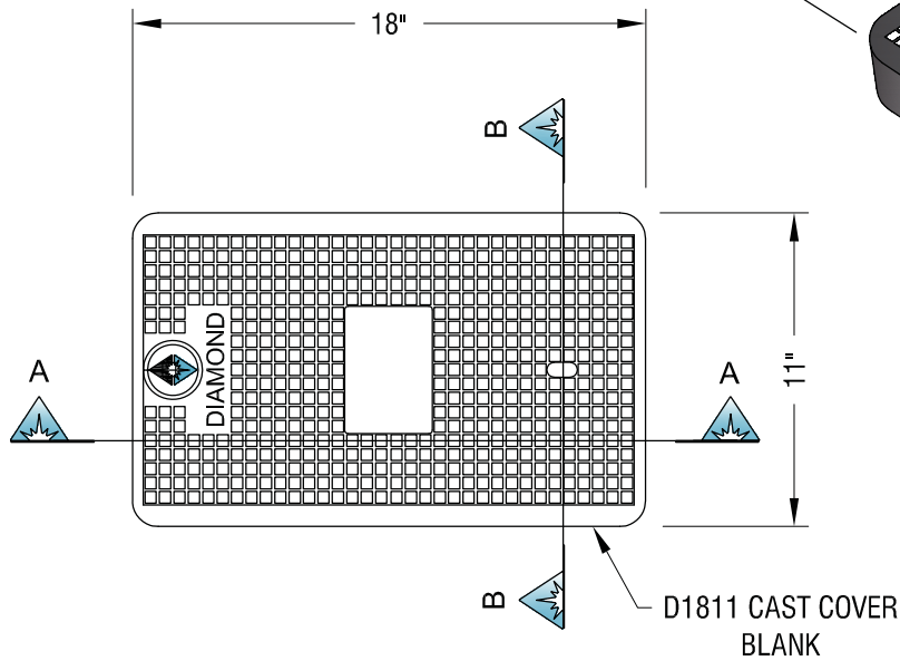
D1811 CAST COVER BLANK SKETCH VIEW
