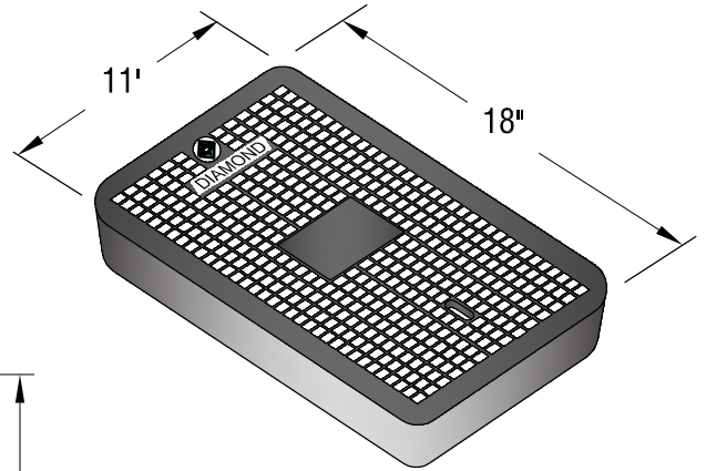
D1811 CAST COVER BLANK SKETCH VIEW
